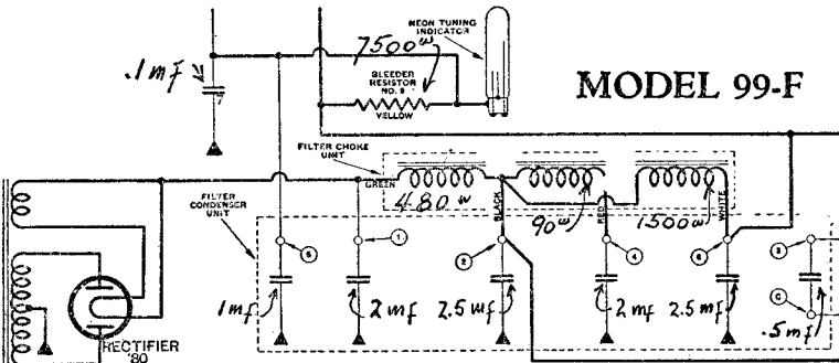
FILTER CIRCUIT OF MODEL 99-F
